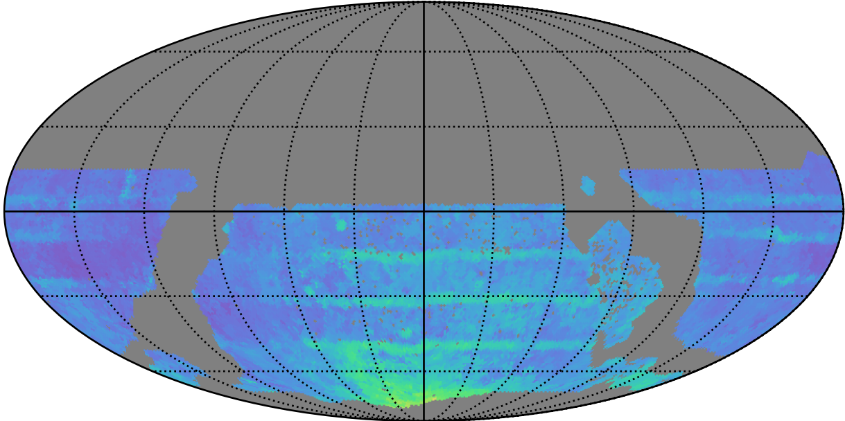
ddf_acor_sf15_lsf30_lsr20_v3.4_10yrs WFD all bands: 80thPercentile Season Length
