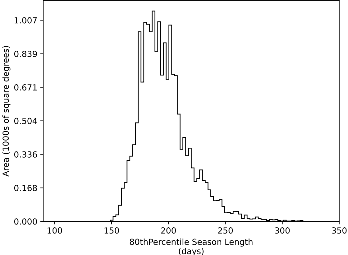
ddf_acor_sf15_lsf30_lsr20_v3.4_10yrs WFD all bands: 80thPercentile Season Length
