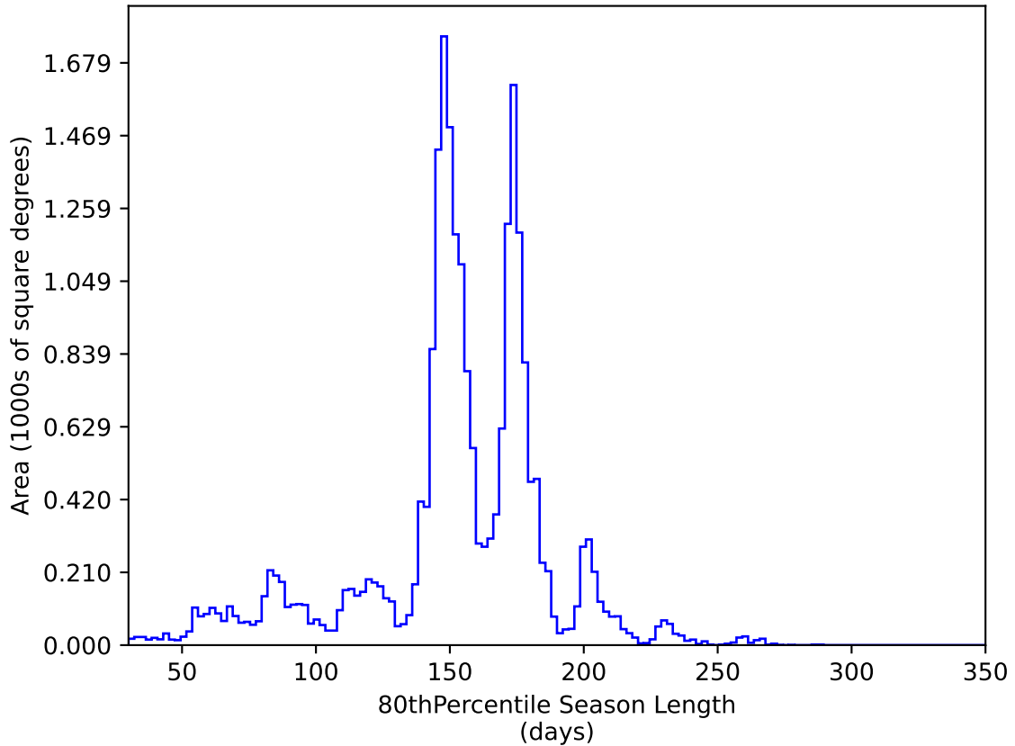
ddf_acor_sf15_lsf30_lsr20_v3.4_10yrs All sky y band: 80thPercentile Season Length
