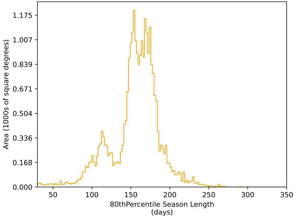
ddf_acor_sf15_lsf30_lsr20_v3.4_10yrs All sky r band: 80thPercentile Season Length
