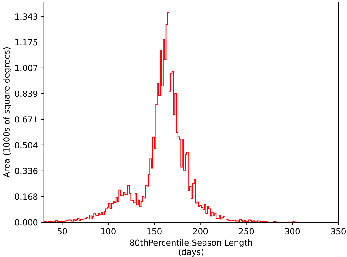
ddf_acor_sf15_lsf30_lsr20_v3.4_10yrs All sky i band: 80thPercentile Season Length
