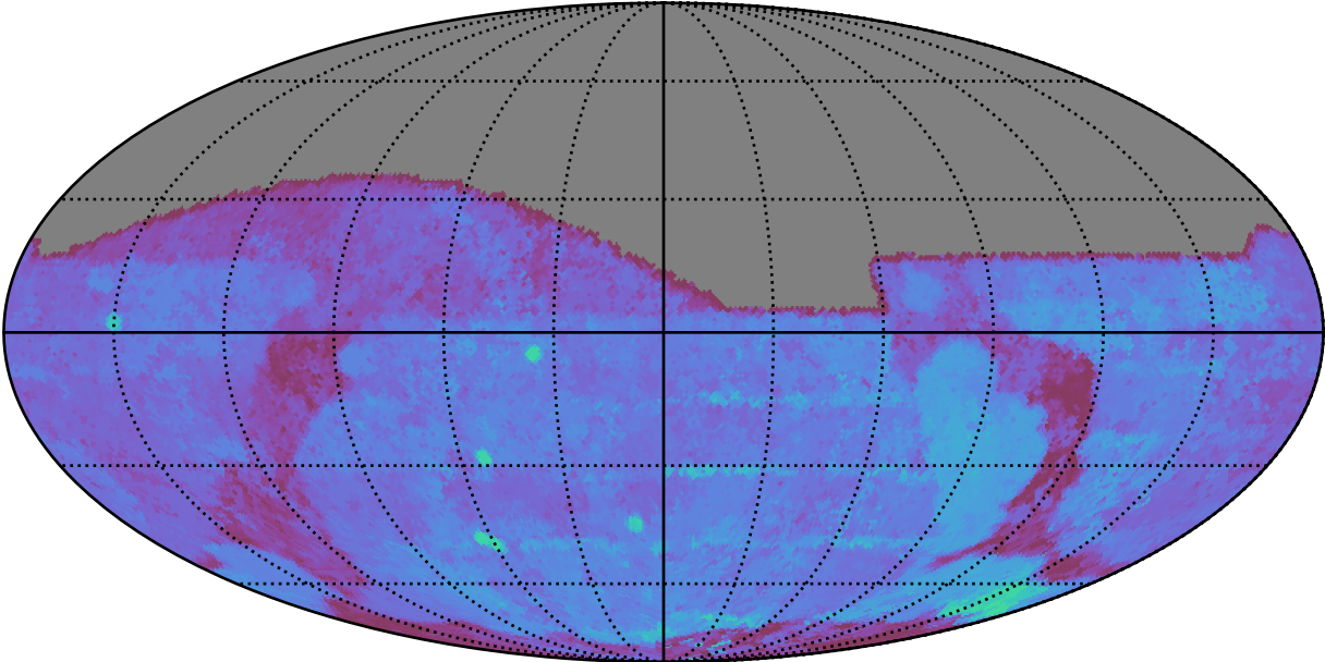
ddf_acor_sf15_lsf30_lsr20_v3.4_10yrs All sky g band: 80thPercentile Season Length
