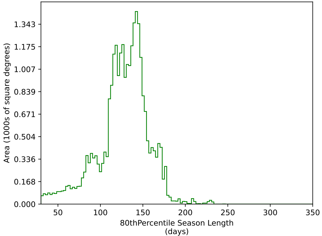
ddf_acor_sf15_lsf30_lsr20_v3.4_10yrs All sky g band: 80thPercentile Season Length
