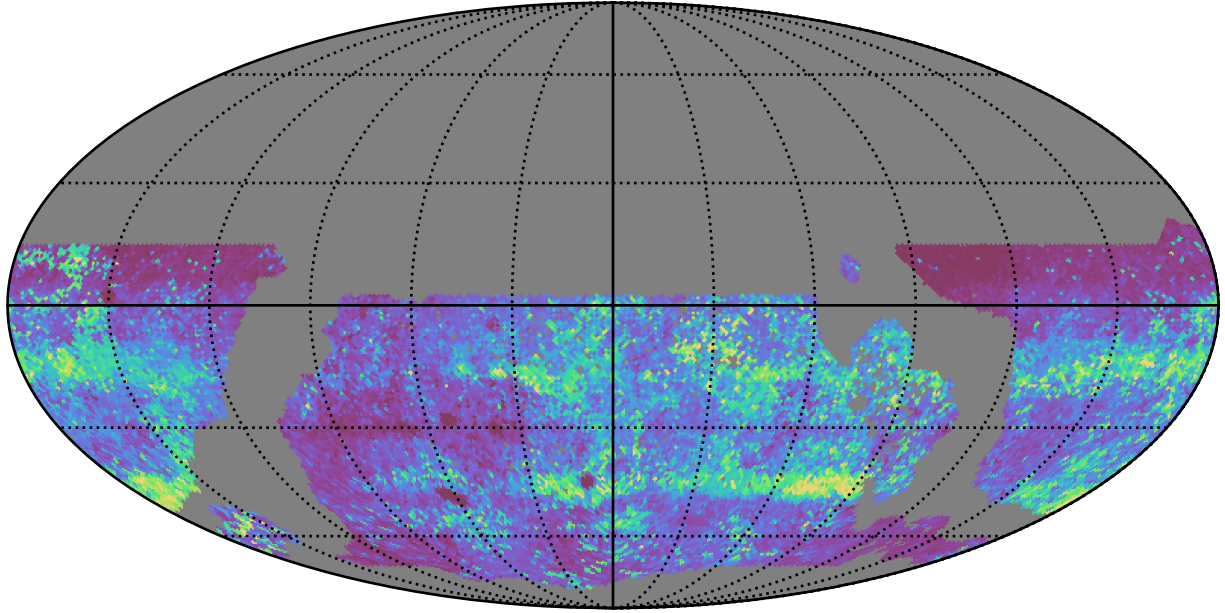
ddf_acor_sf15_lsf30_lsr20_v3.4_10yrs WFD zy bands: 75th Percentile Intranight Timespan
