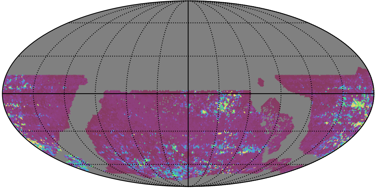
ddf_acor_sf15_lsf30_lsr20_v3.4_10yrs WFD z band: 75th Percentile Intranight Timespan
