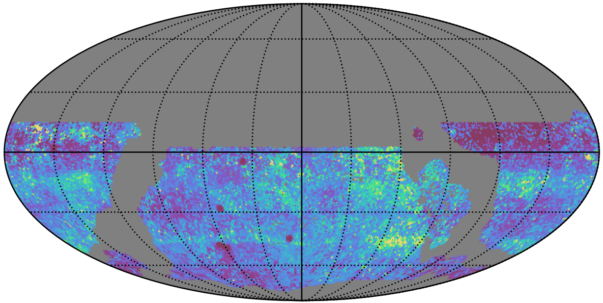
ddf_acor_sf15_lsr30_lsr20_v3.4_10yrs WFD y band: 75th Percentile Intranight Timespan
