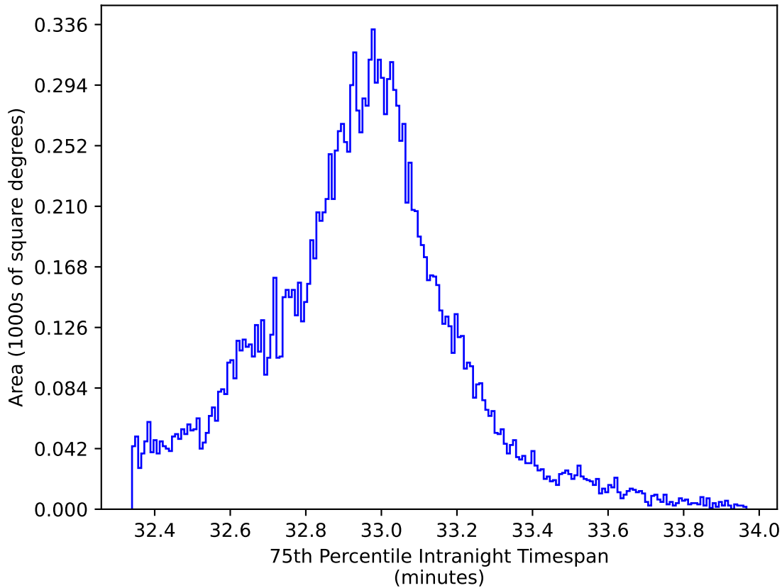
ddf_acor_sf15_lsf30_lsr20_v3.4_10yrs WFD y band: 75th Percentile Intranight Timespan
