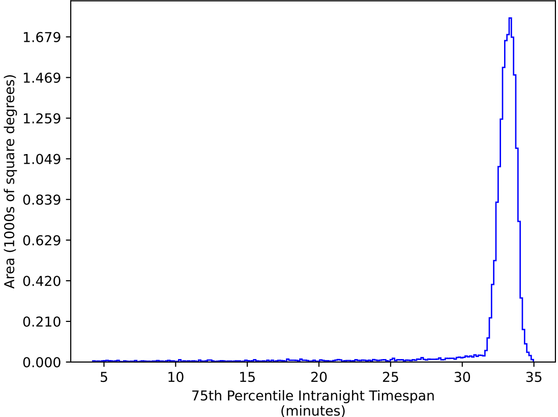
ddf_acor_sf15_lsf30_lsr20_v3.4_10yrs WFD ug bands: 75th Percentile Intranight Timespan
