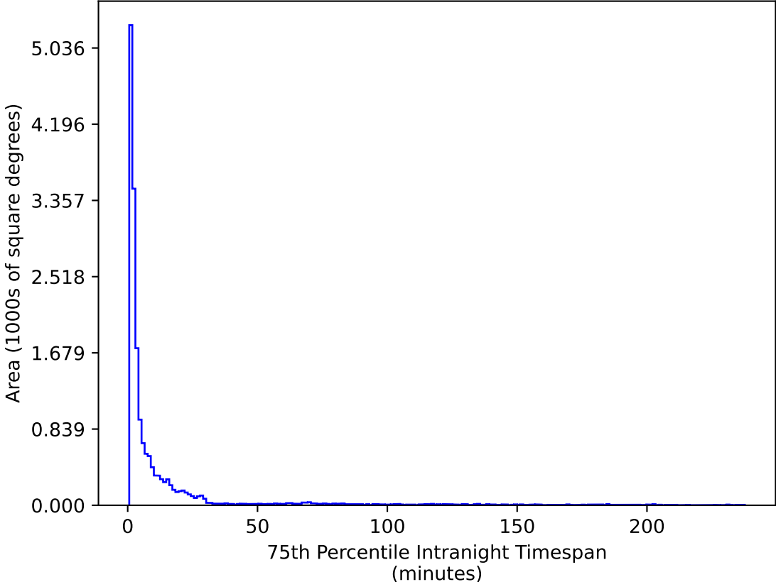
ddf_acor_sf15_lsf30_lsr20_v3.4_10yrs WFD u band: 75th Percentile Intranight Timespan
