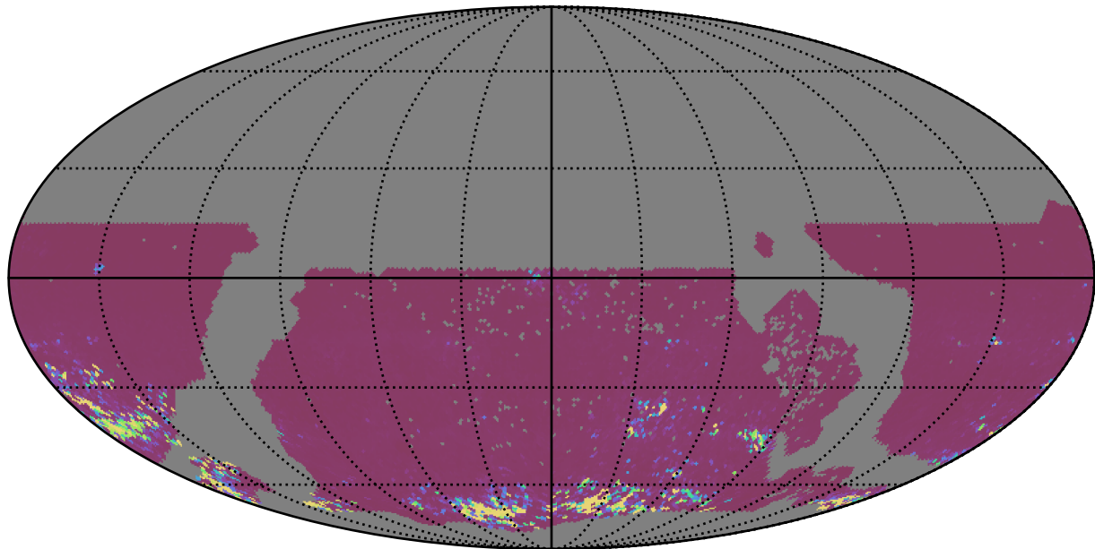
ddf_acor_sf15_lsf30_lsr20_v3.4_10yrs WFD ri bands: 75th Percentile Intranight Timespan
