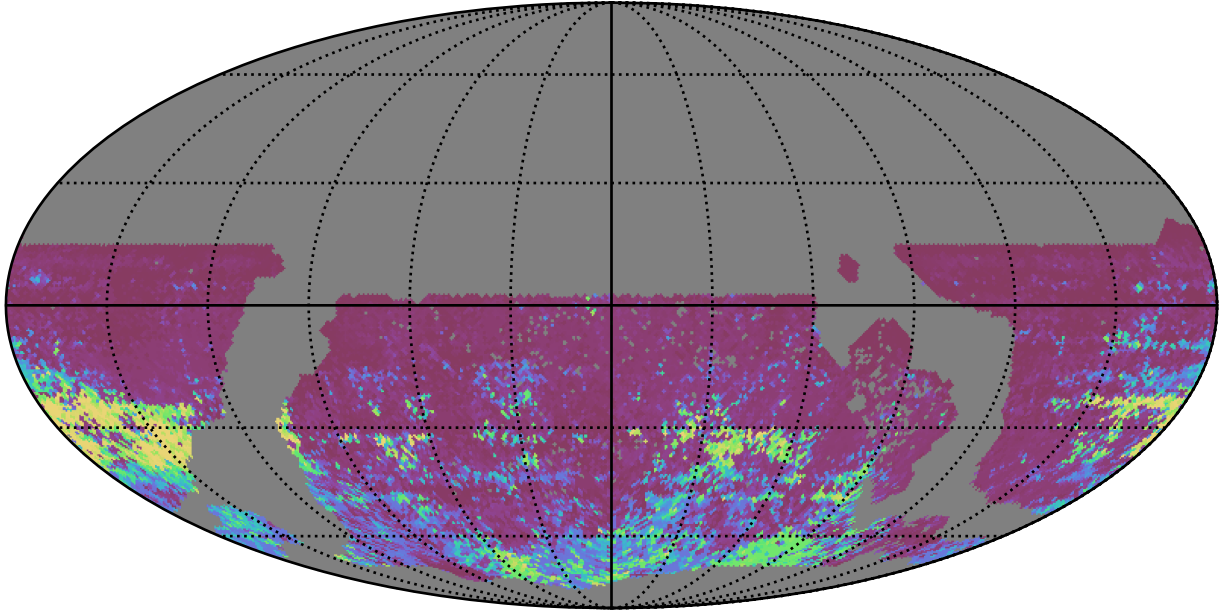
ddf_acor_sf15_lsf30_lsr20_v3.4_10yrs WFD r band: 75th Percentile Intranight Timespan
