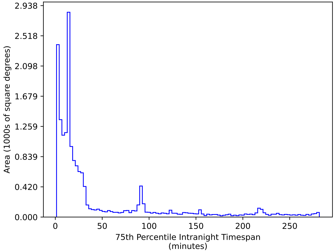
ddf_acor_sf15_lsf30_lsr20_v3.4_10yrs WFD r band: 75th Percentile Intranight Timespan
