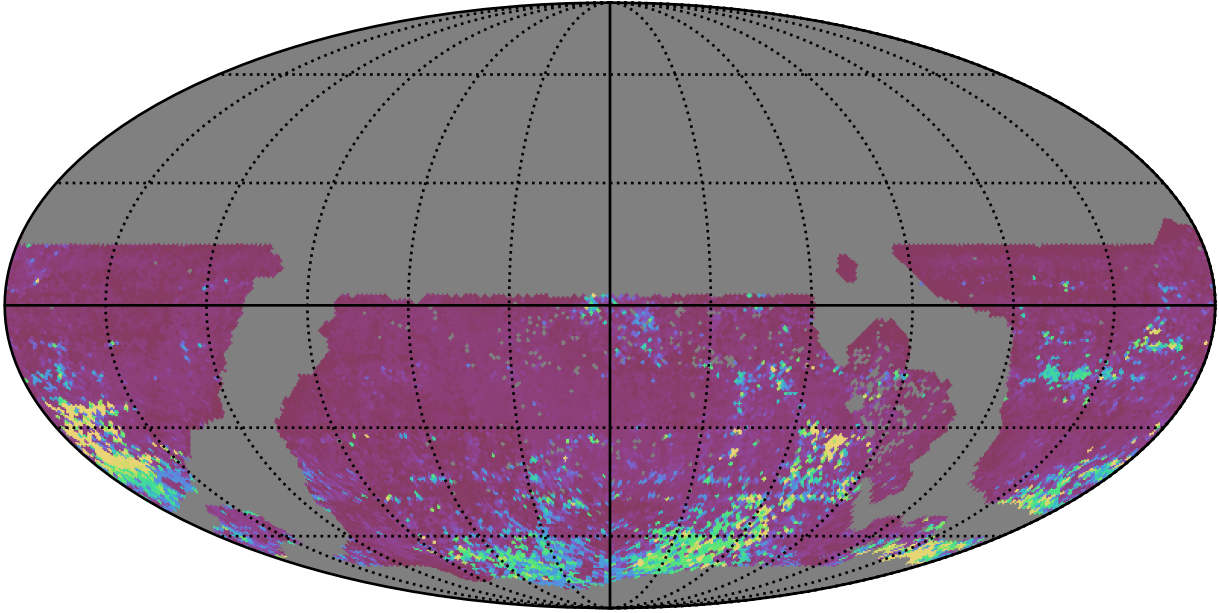
ddf_acor_sf15_lsf30_lsr20_v3.4_10yrs WFD i band: 75th Percentile Intranight Timespan
