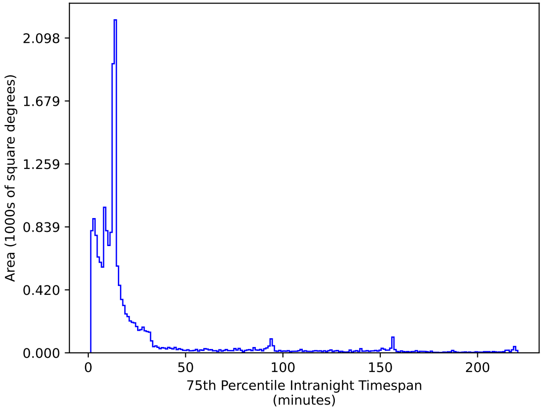
ddf_acor_sf15_lsf30_lsr20_v3.4_10yrs WFD i band: 75th Percentile Intranight Timespan
