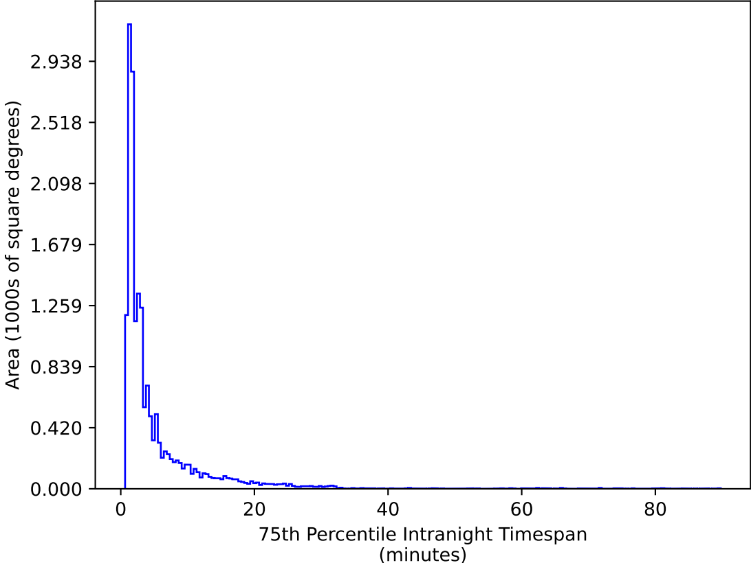
ddf_acor_sf15_lsf30_lsr20_v3.4_10yrs WFD g band: 75th Percentile Intranight Timespan
