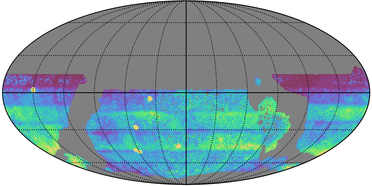
ddf_acor_sf15_lsf30_lsr20_v3.4_10yrs WFD all bands: 75th Percentile Intranight Timespan
