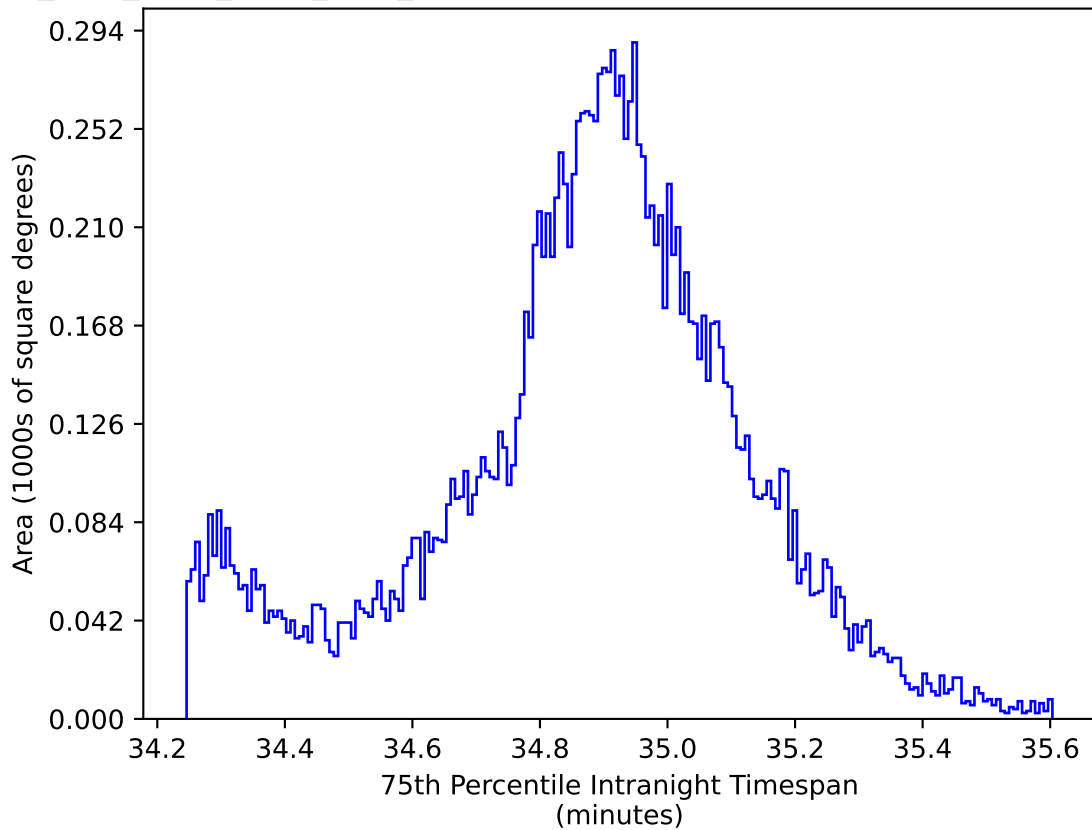
ddf_acor_sf15_lsf30_lsr20_v3.4_10yrs WFD all bands: 75th Percentile Intranight Timespan
