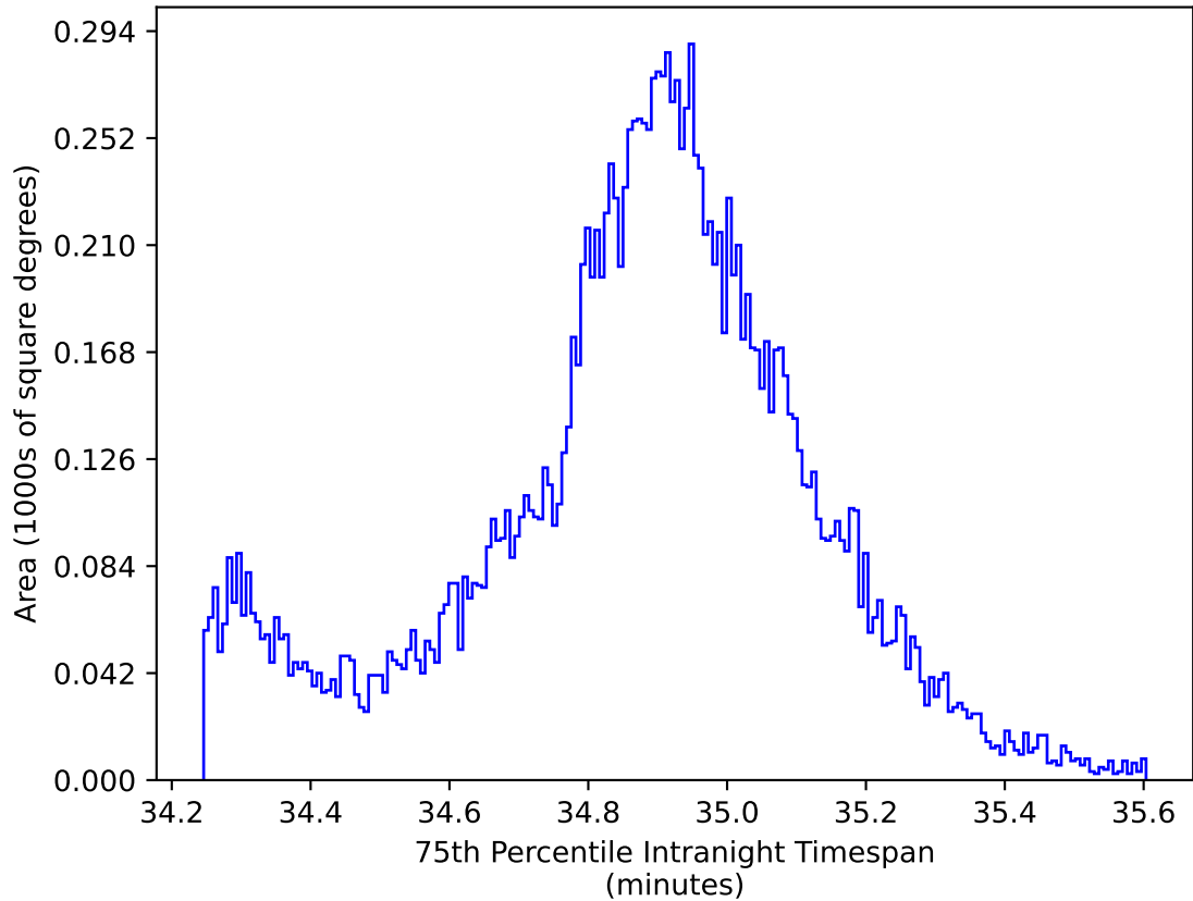
ddf_acor_sf15_lsf30_lsr20_v3.4_10yrs WFD: 75th Percentile Intranight Timespan
