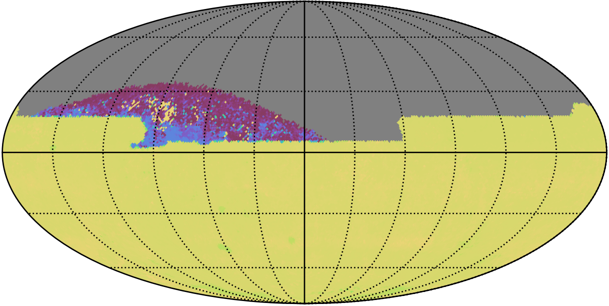
ddf_acor_sf15_lsf30_lsr20_v3.4_10yrs All sky zy bands: 75th Percentile Intranight Timespan
