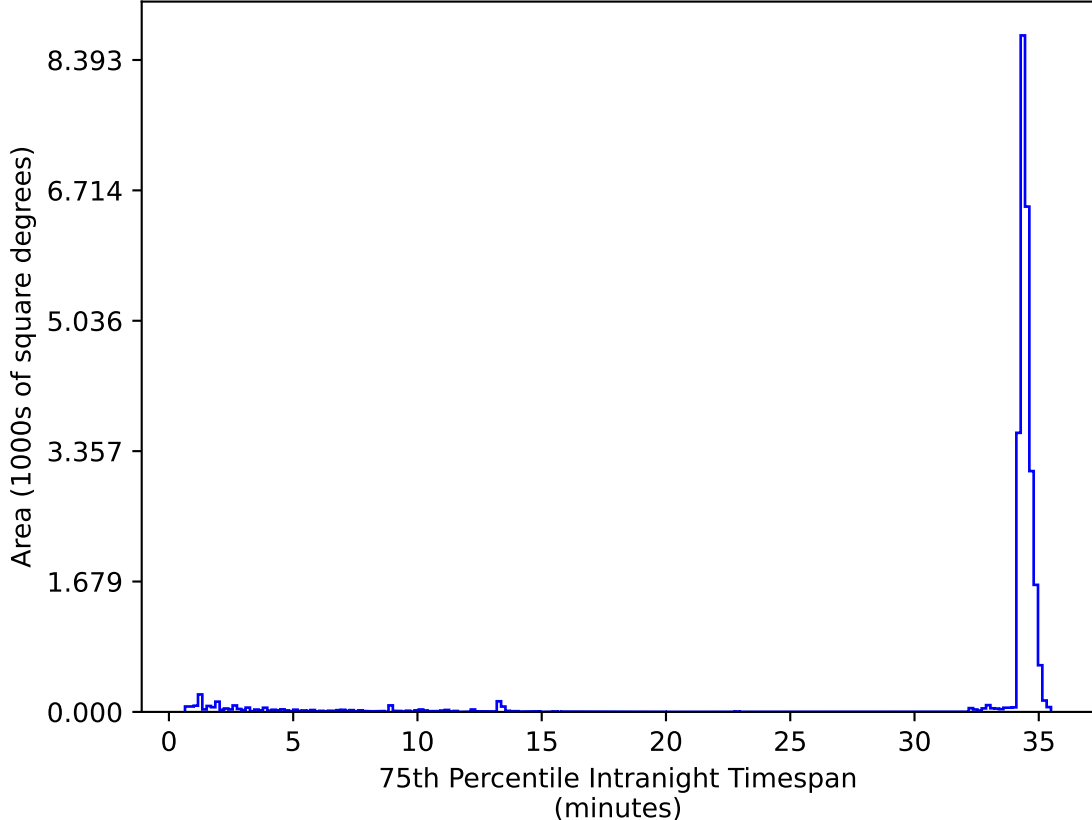
ddf_acor_sf15_lsf30_lsr20_v3.4_10yrs All sky zy bands: 75th Percentile Intranight Timespan
