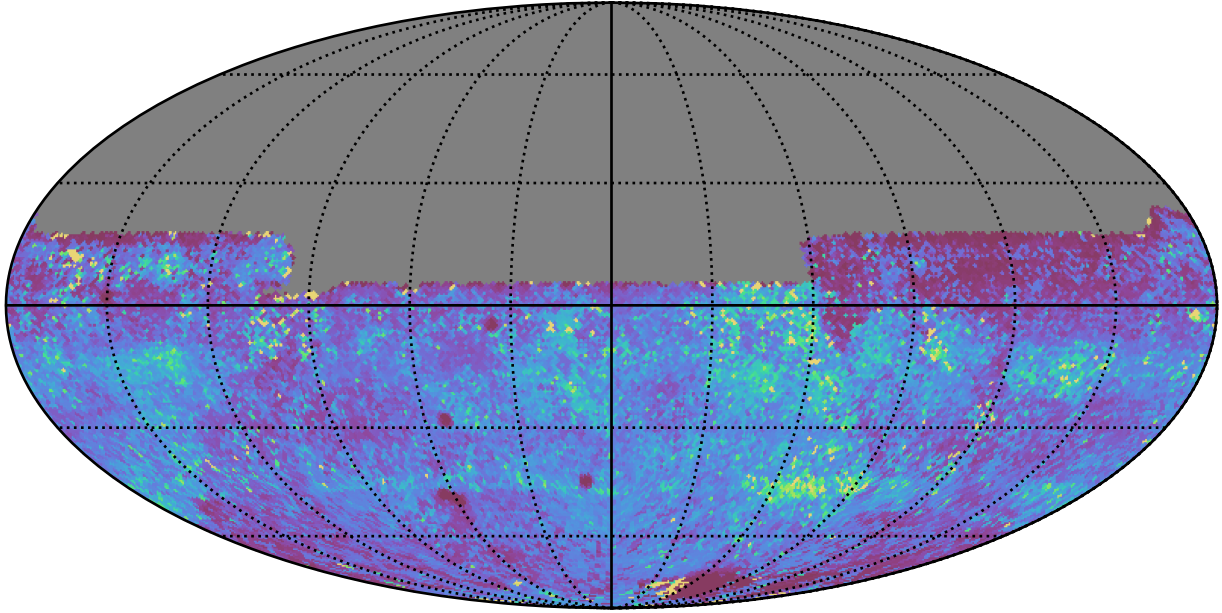
ddf_acor_sf15_lsf30_lsr20_v3.4_10yrs All sky y band: 75th Percentile Intranight Timespan
