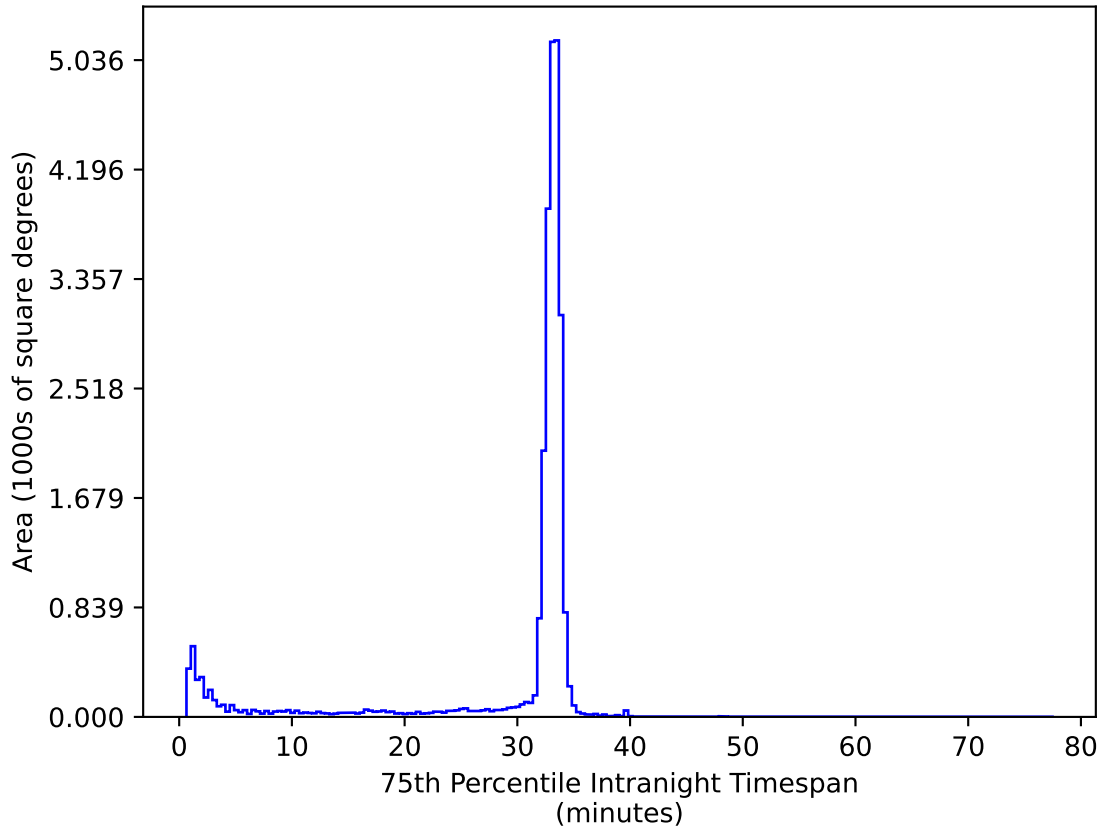
ddf_acor_sf15_lsf30_lsr20_v3.4_10yrs All sky ug bands: 75th Percentile Intranight Timespan
