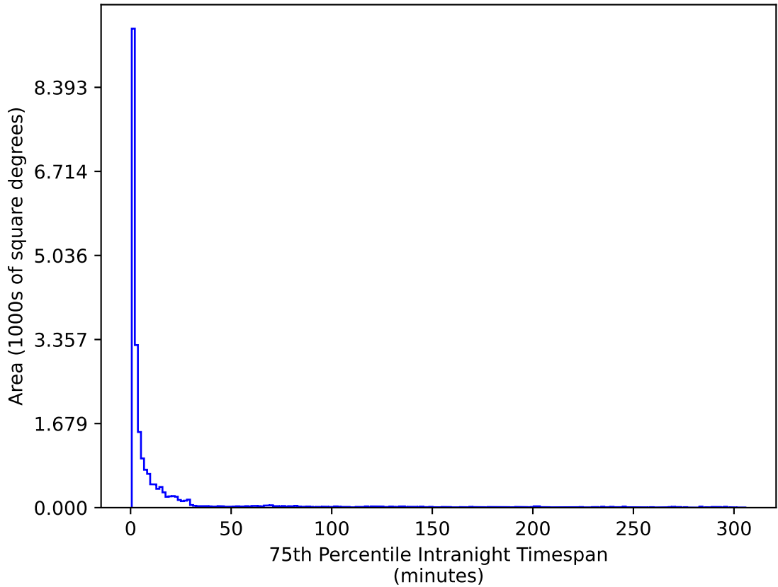
ddf_acor_sf15_lsf30_lsr20_v3.4_10yrs All sky u band: 75th Percentile Intranight Timespan
