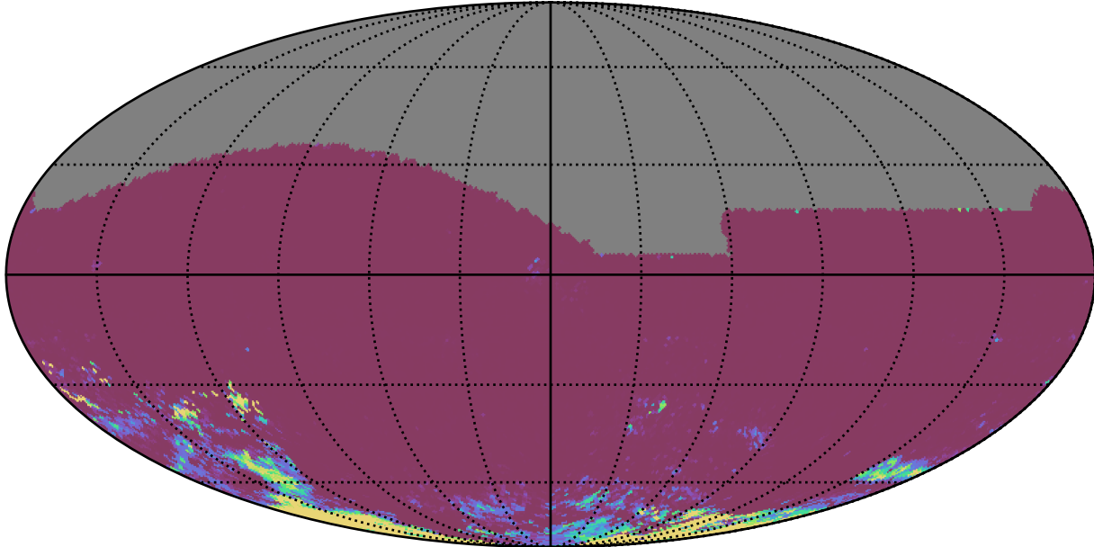
ddf_acor_sf15_lsf30_lsr20_v3.4_10yrs All sky ri bands: 75th Percentile Intranight Timespan
