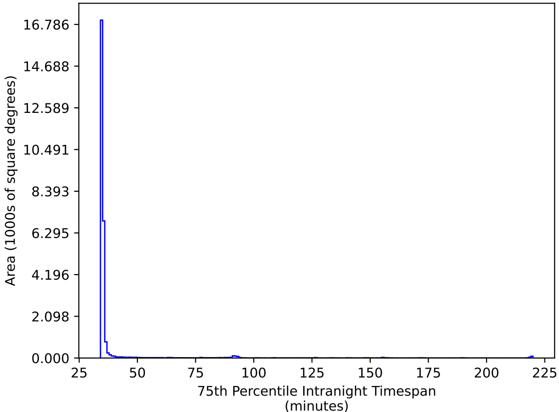
ddf_acor_sf15_lsf30_lsr20_v3.4_10yrs All sky ri bands: 75th Percentile Intranight Timespan
