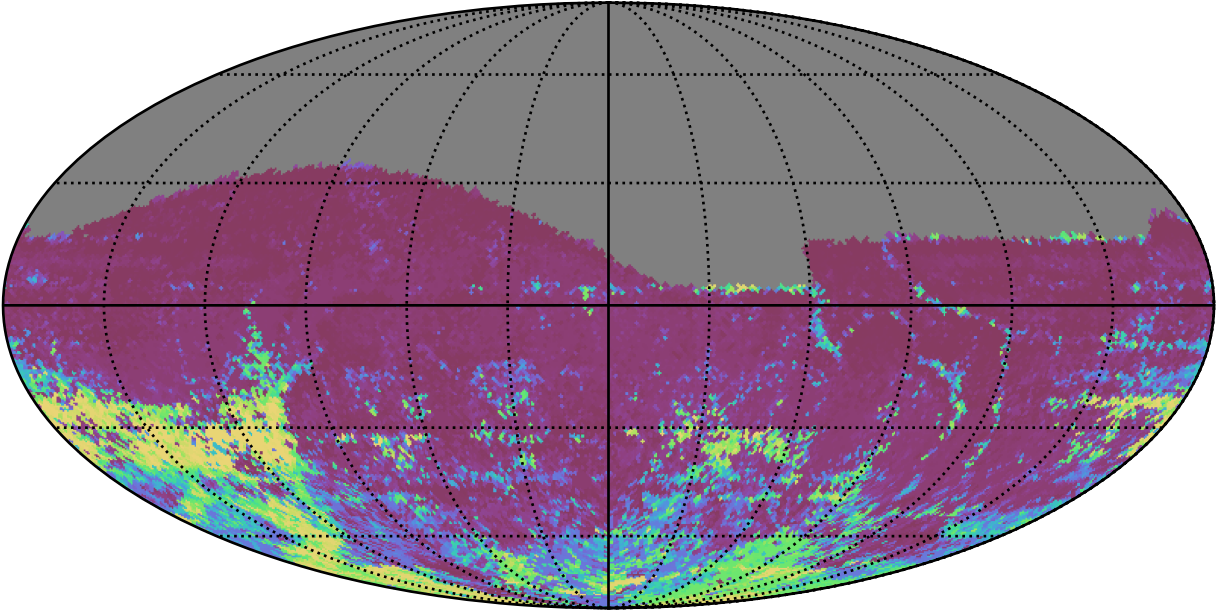
ddf_acor_sf15_lsf30_lsr20_v3.4_10yrs All sky r band: 75th Percentile Intranight Timespan
