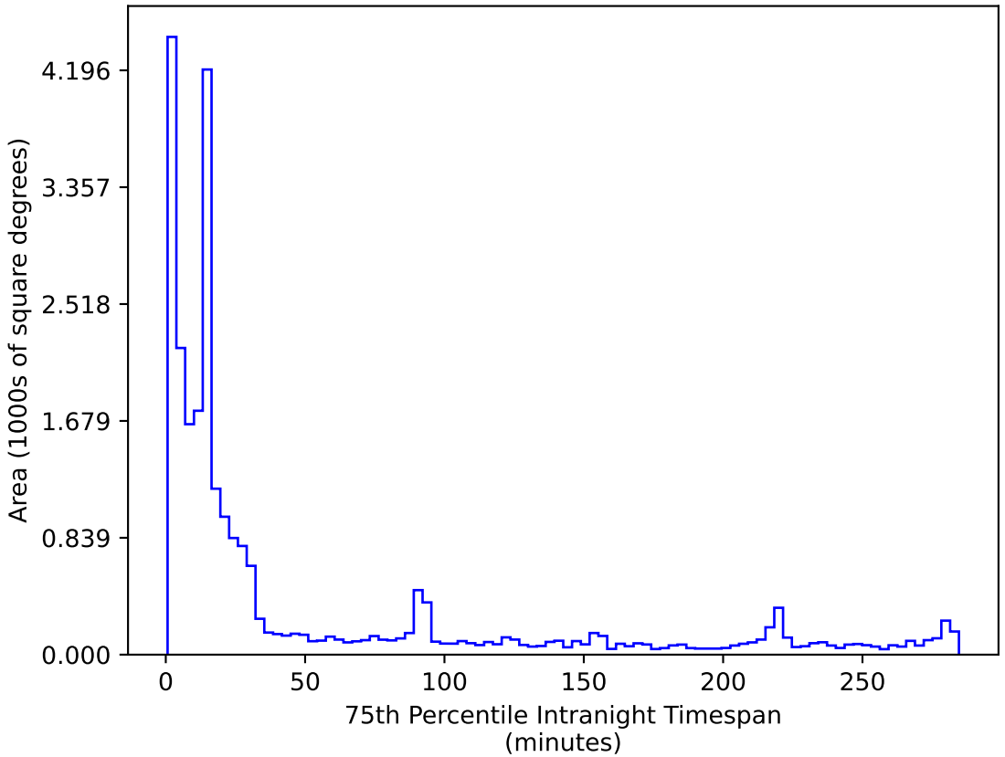
ddf_acor_sf15_lsf30_lsr20_v3.4_10yrs All sky r band: 75th Percentile Intranight Timespan
