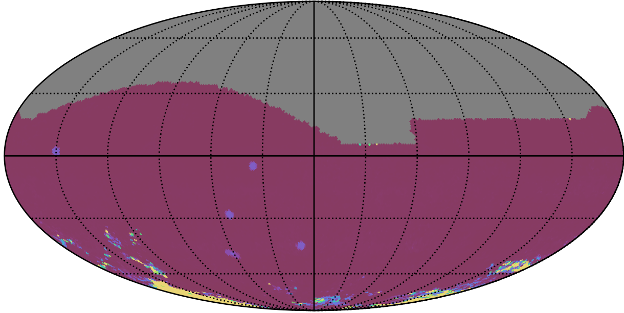
ddf_acor_sf15_lsf30_lsr20_v3.4_10yrs All sky iz bands: 75th Percentile Intranight Timespan
