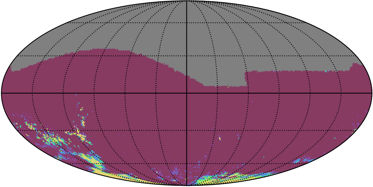
ddf_acor_sf15_lsf30_lsr20_v3.4_10yrs All sky gr bands: 75th Percentile Intranight Timespan
