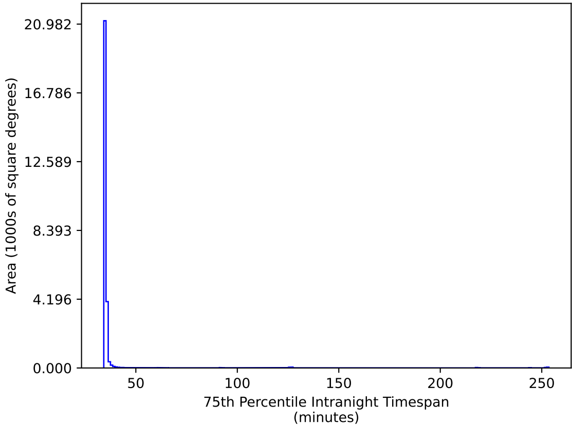
ddf_acor_sf15_lsf30_lsr20_v3.4_10yrs All sky gr bands: 75th Percentile Intranight Timespan
