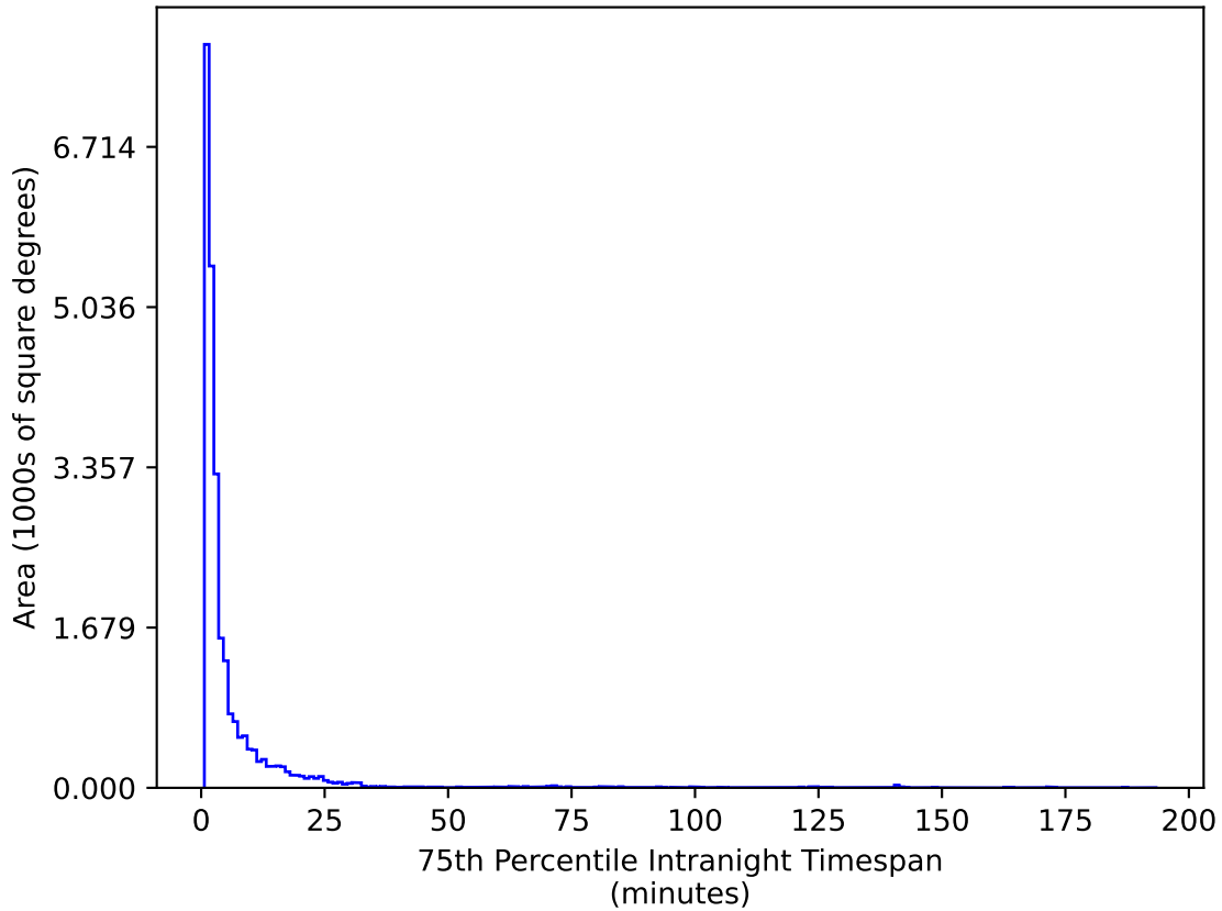
ddf_acor_sf15_lsf30_lsr20_v3.4_10yrs All sky g band: 75th Percentile Intranight Timespan
