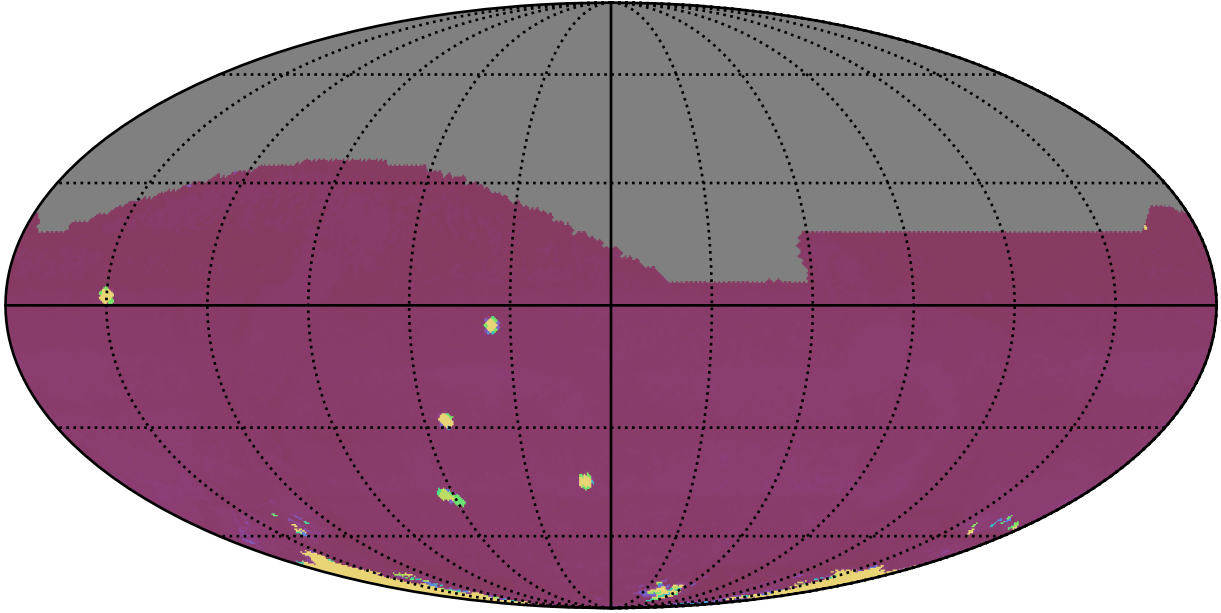
ddf_acor_sf15_lsf30_lsr20_v3.4_10yrs All sky all bands: 75th Percentile Intranight Timespan
