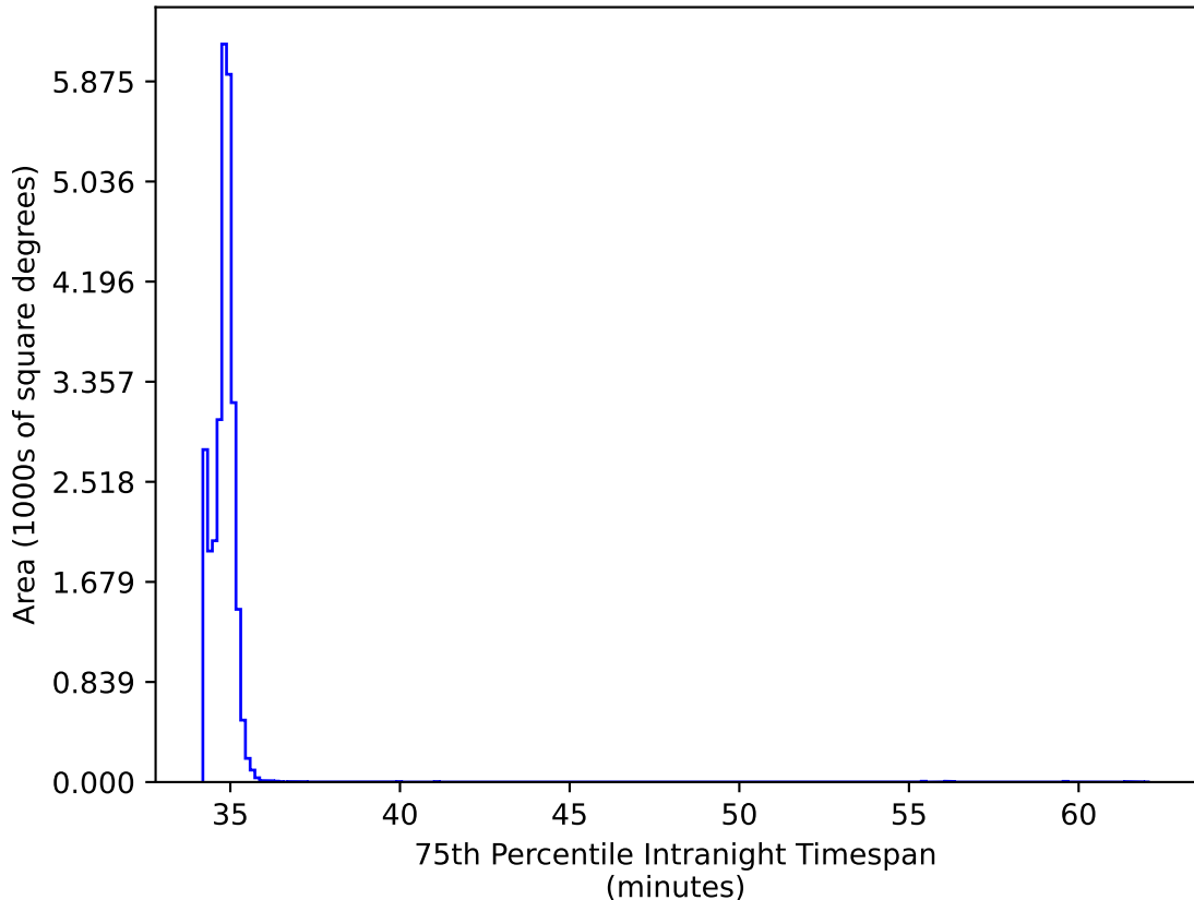
ddf_acor_sf15_lsf30_lsr20_v3.4_10yrs All sky all bands: 75th Percentile Intranight Timespan
