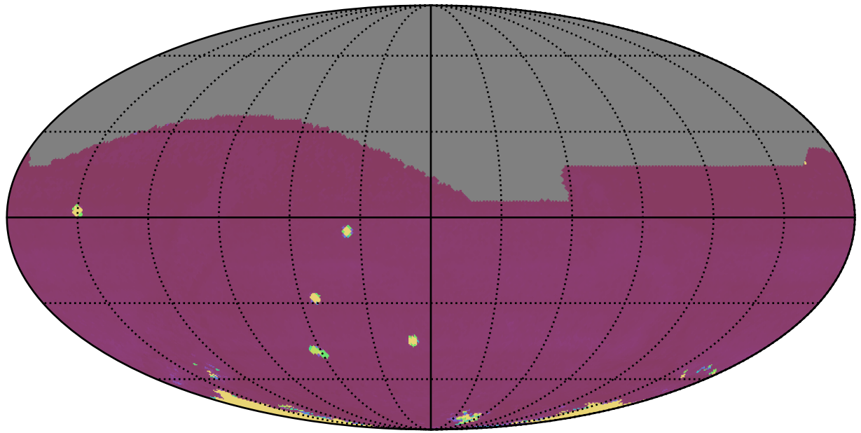
ddf_acor_sf15_lsf30_lsr20_v3.4_10yrs All sky: 75th Percentile Intranight Timespan
