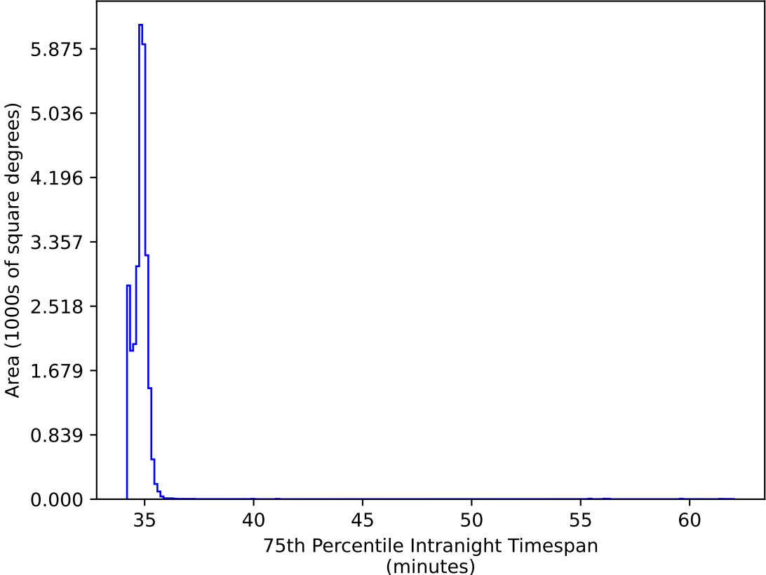
ddf_acor_sf15_lsf30_lsr20_v3.4_10yrs All sky: 75th Percentile Intranight Timespan
