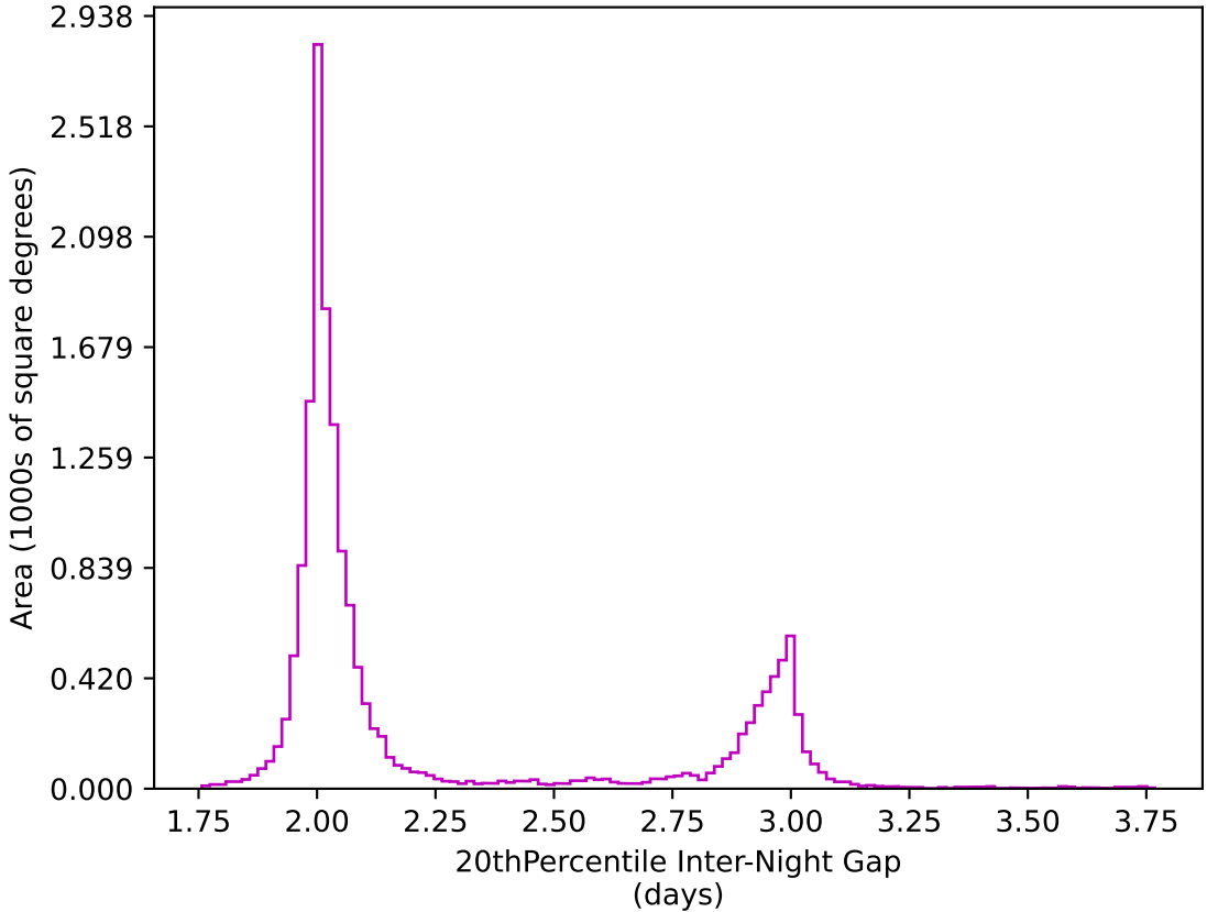
ddf_acor_sf15_lsf30_lsr20_v3.4_10yrs WFD z band: 20thPercentile Inter-Night Gap
