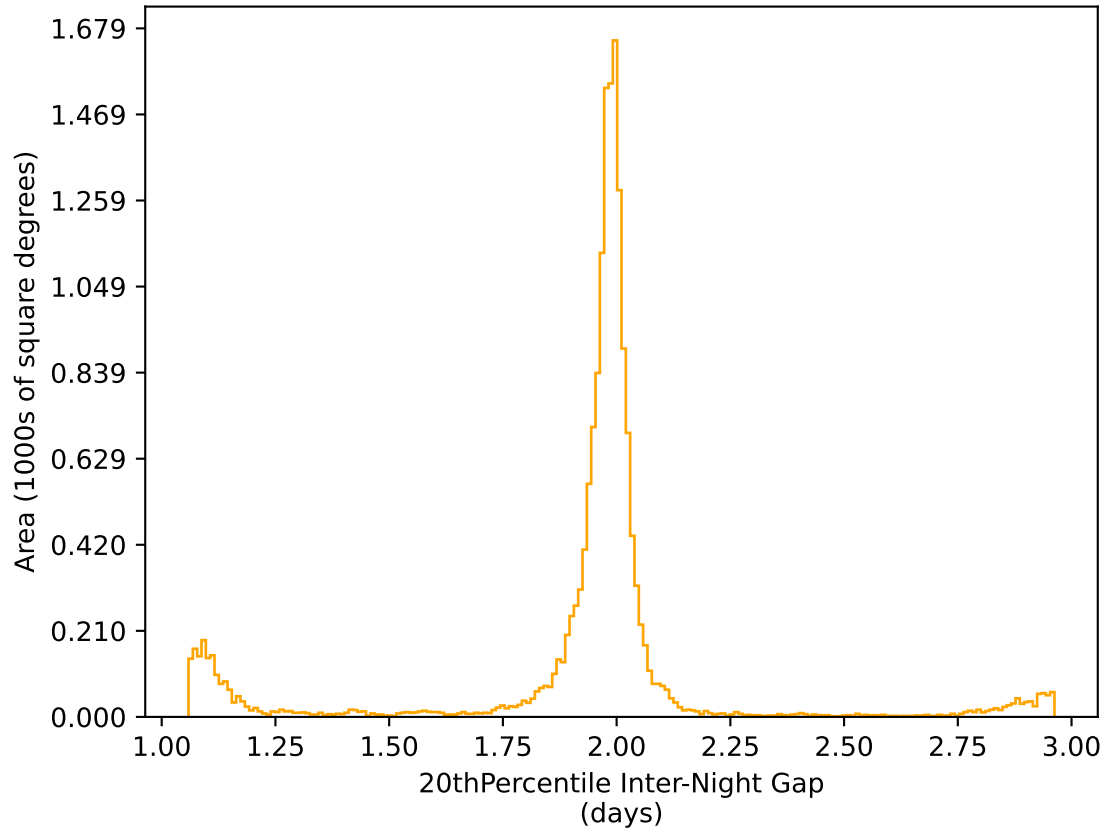
ddf_acor_sf15_lsf30_lsr20_v3.4_10yrs WFD r band: 20thPercentile Inter-Night Gap
