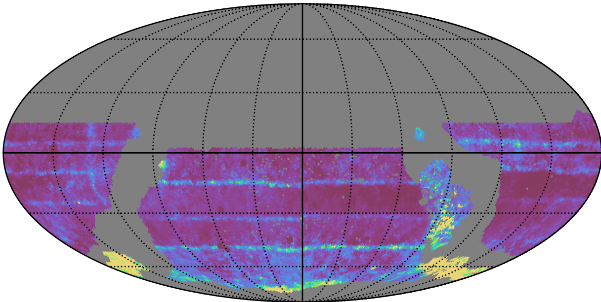
ddf_acor_sf15_lsf30_lsr20_v3.4_10yrs WFD all bands: 20thPercentile Inter-Night Gap
