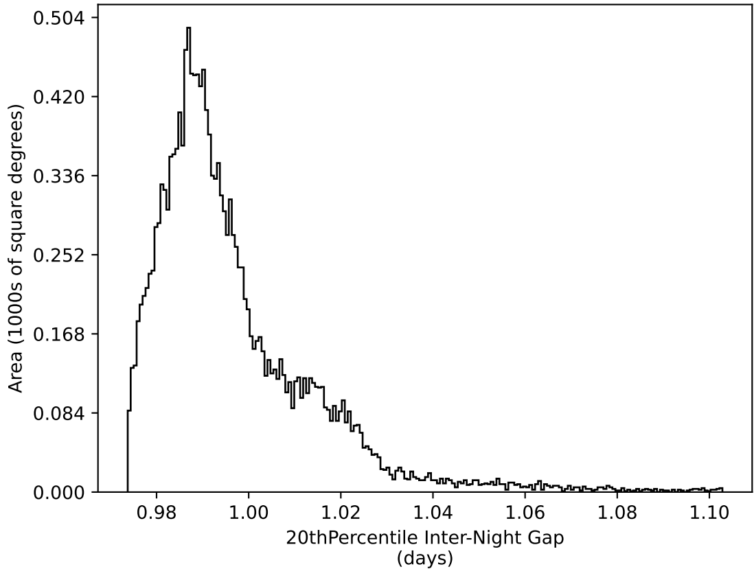
ddf_acor_sf15_lsf30_lsr20_v3.4_10yrs WFD all bands: 20thPercentile Inter-Night Gap
