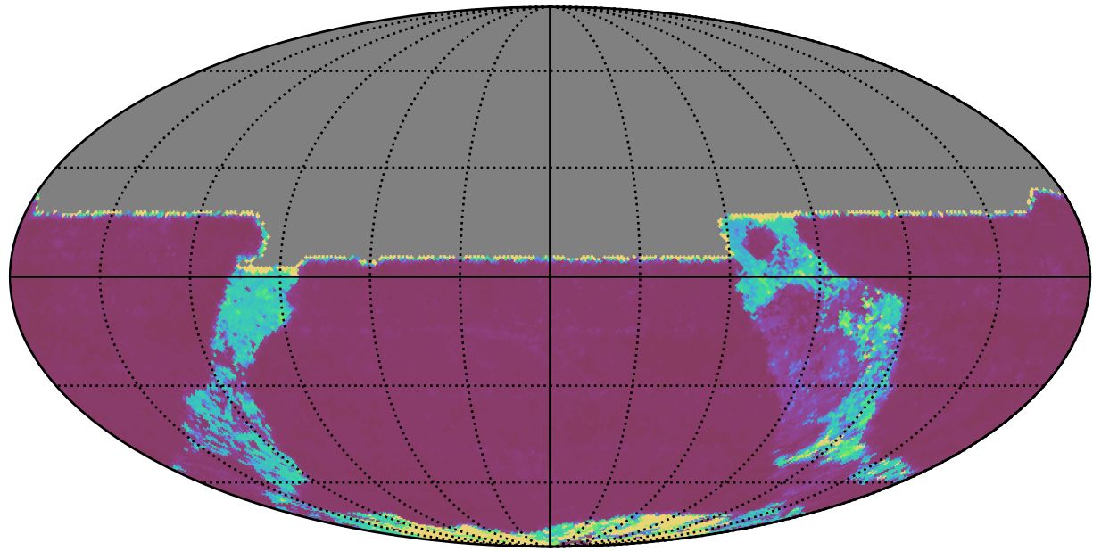
ddf_acor_sf15_lsf30_lsr20_v3.4_10yrs All sky y band: 20thPercentile Inter-Night Gap
