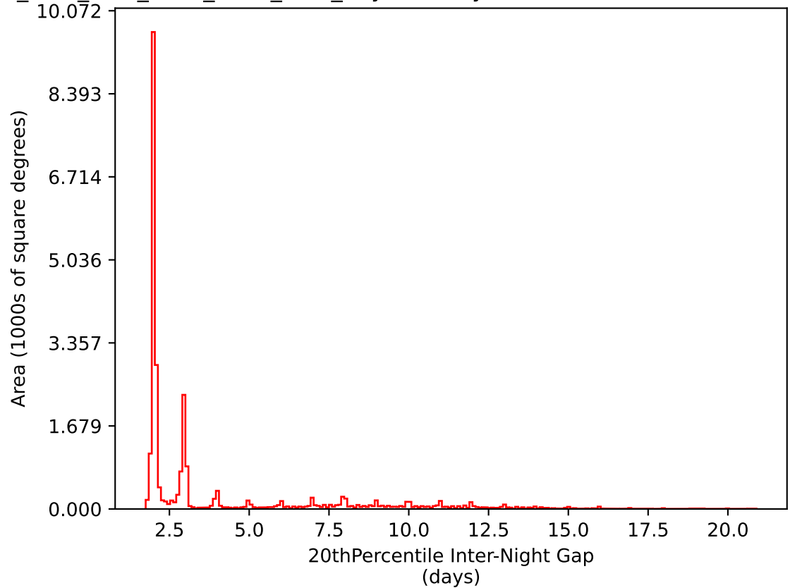
ddf_acor_sf15_lsf30_lsr20_v3.4_10yrs All sky i band: 20thPercentile Inter-Night Gap
