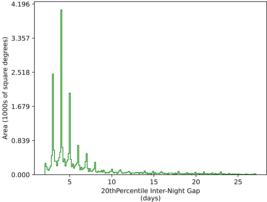
ddf_acor_sf15_lsf30_lsr20_v3.4_10yrs All sky g band: 20thPercentile Inter-Night Gap
