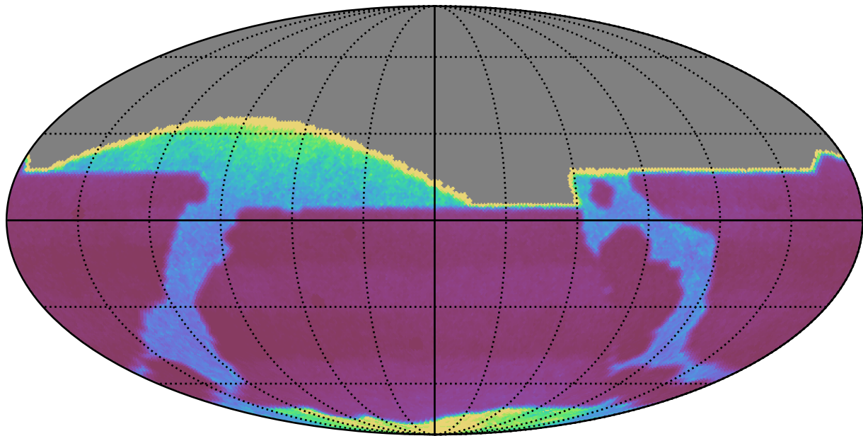
ddf_acor_sf15_lsf30_lsr20_v3.4_10yrs : properMotion
