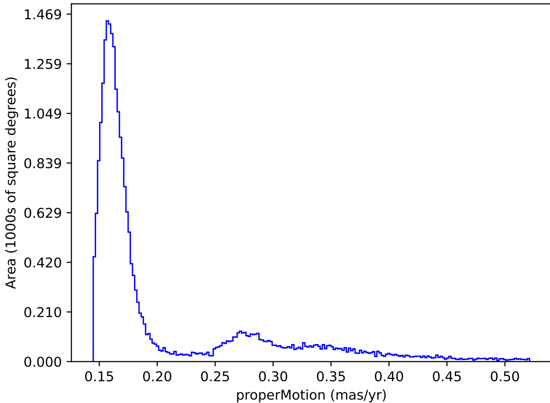
ddf_acor_sf15_lsf30_lsr20_v3.4_10yrs : properMotion
