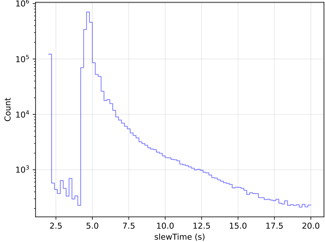
ddf_acor_sf15_Isf30_Isr20_v3.4_10yrs All visits: Zoom Slew Time Histogram
