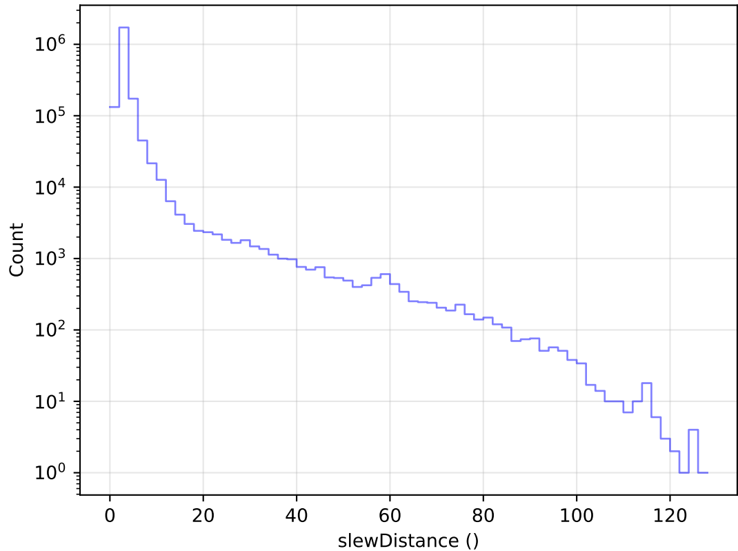
ddf_acor_sf15_lsf30_lsr20_v3.4_10yrs All visits: Slew Distance Histogram
